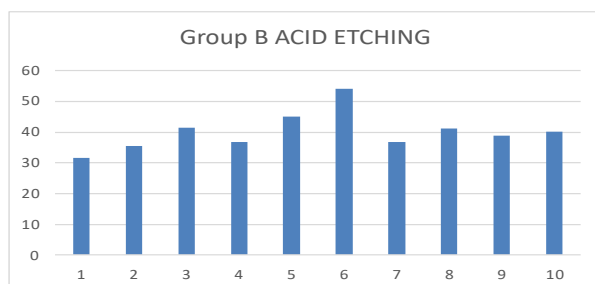
Graph 2: Dislodgement force in N for Group B Acid etching
