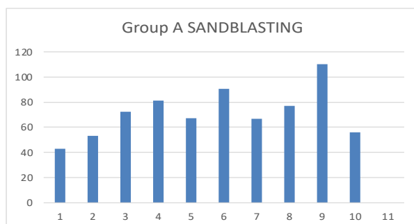
Graph 1 : Dislodgement force in N for Group A Sandblasting
